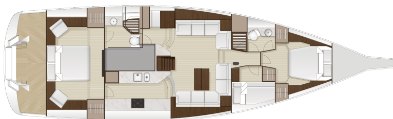
Lower Deck
